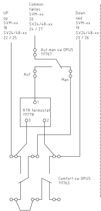
Room thermostat +Aut/man Switch Opus (Jumper original pos.)
