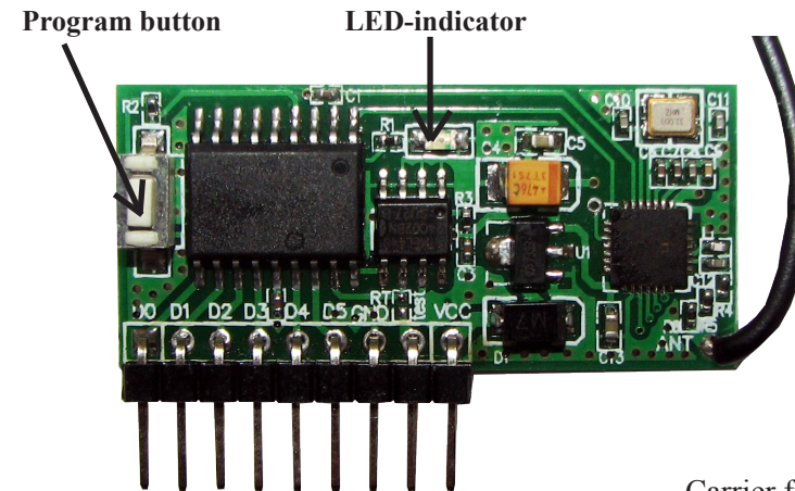
Carrier frequency 868 MHz Battery 12V/33 mA type LRV08L
